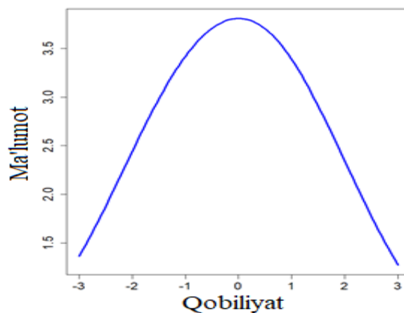
4-rasm. Test ma'lumoti chizig'i
